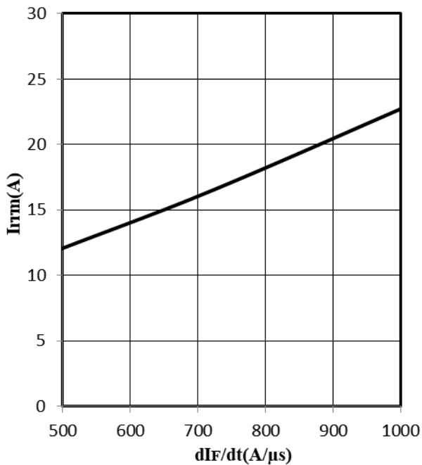
Fig 19. Typical I_{rrm} as a function of dI_F/dt ( I_F=30A )
