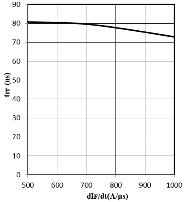
Fig 18. Typical t_{rr} as a function of dI_F/dt ( I_F=30A )
