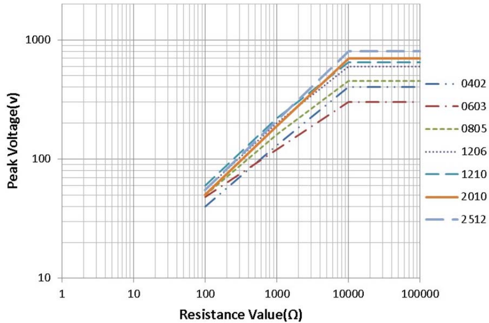
10/700µs Single-pulse high-voltage overload test
